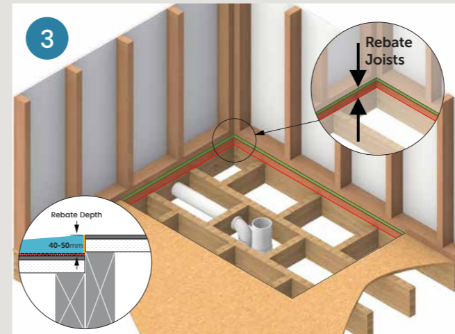
3 Rebate joists to required depth to suit base model Fix additional joists to support ply infill
