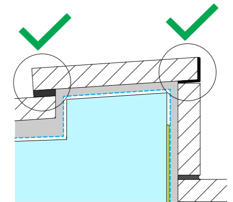
Concrete Floor - Mix tile adhesive and apply with trowel up to outlined base area. 8 hour cure time
