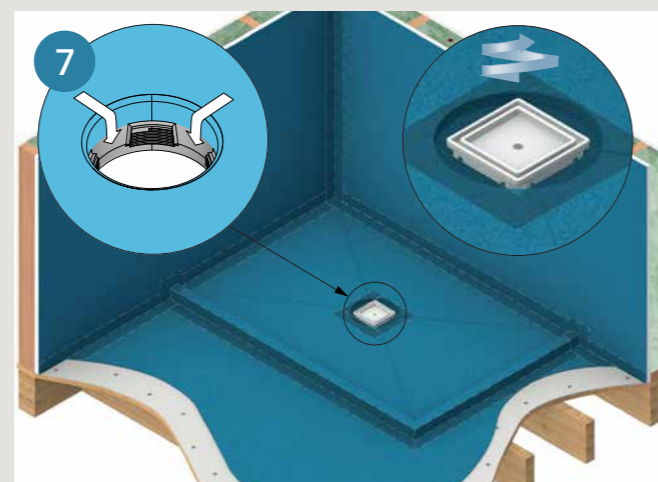
Apply butyl tapes and waterproof floor and walls. Screw the centre drain tile insert component into the LM flange
