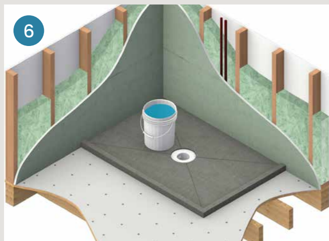
Fit Solaire® base and weigh down with adhesive pale filled with water
