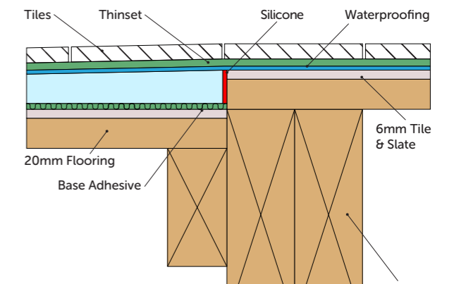
Rebate joists to required depth to suit base model Fix additional joists to support ply infill
