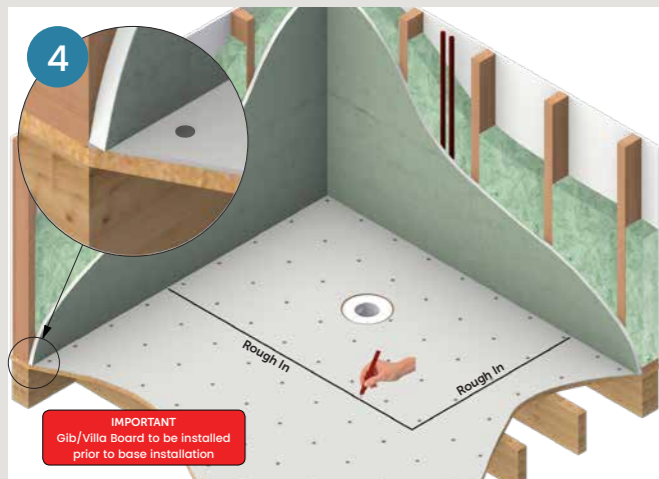
Install Gib/Villa board walls ensuring it is installed down to floor substrate. Dry fit base and mark outline shape on floor
