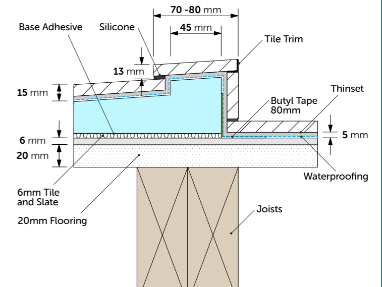
Concrete Floor - Mix tile adhesive and apply with trowel up to outlined base area. 8 hour cure time
