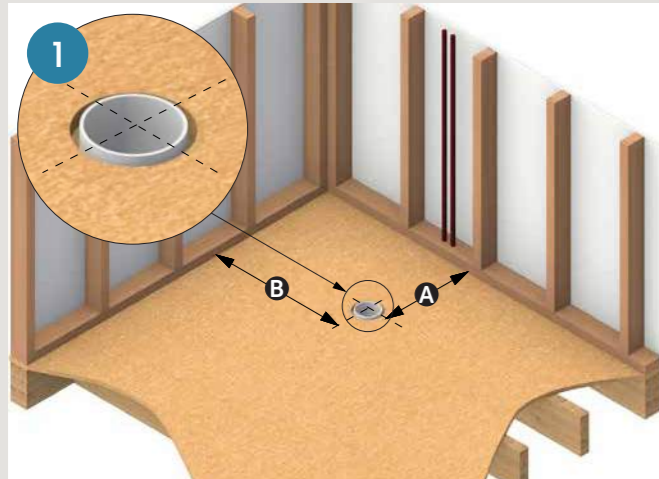
Install PVC drain pipe through sub floor, for (A) & (B) set out dimensions off studs refer to Rough-In Guide
