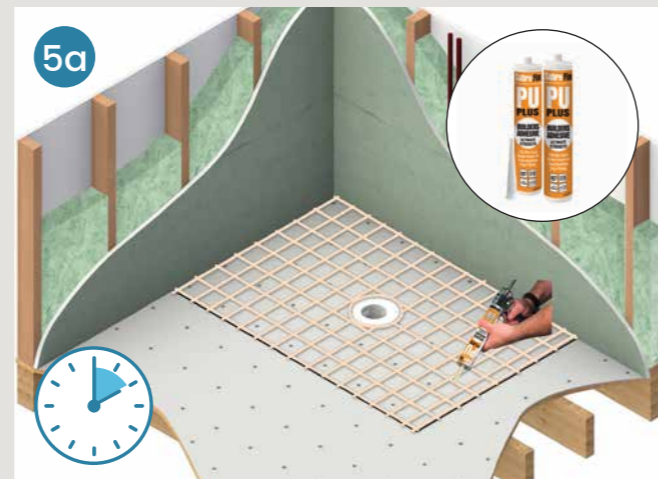
Tile and Slate Floor - Apply polyurethane adhesive. 2 hour cure time (Adhesive Kit included)
