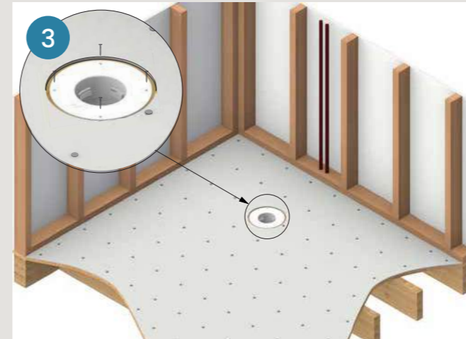
Install liquid membrane flange to PVC drain and secure to sub floor
