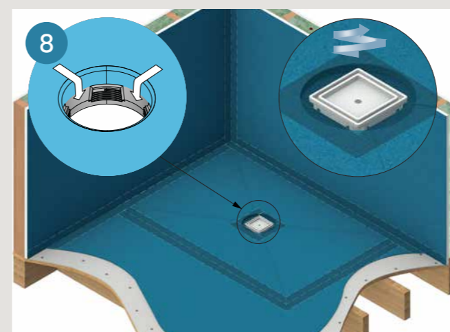
8 Apply butyl tapes and waterproof floors and walls. Screw the centre drain tile insert component into the LM flange
