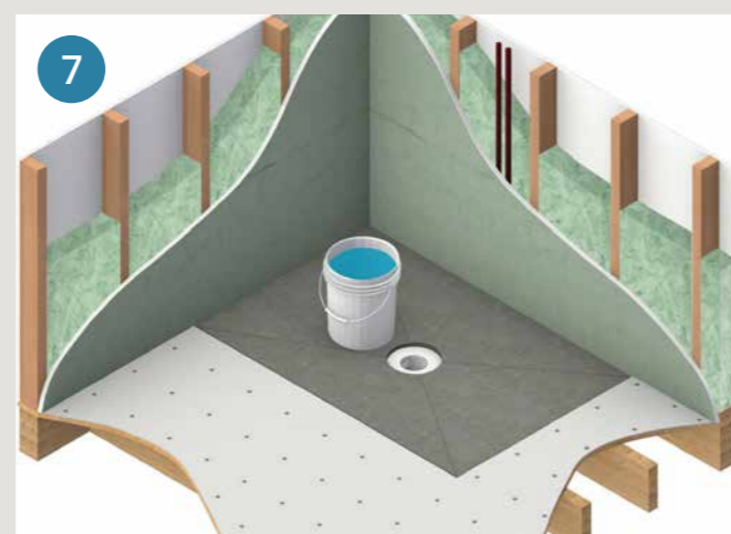
7 Fit Solaire® base and weigh down with adhesive pallet filled with water
