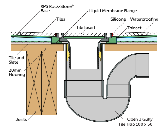
Rebate joists to required depth to suit base model Fix additional joists to support ply infill
