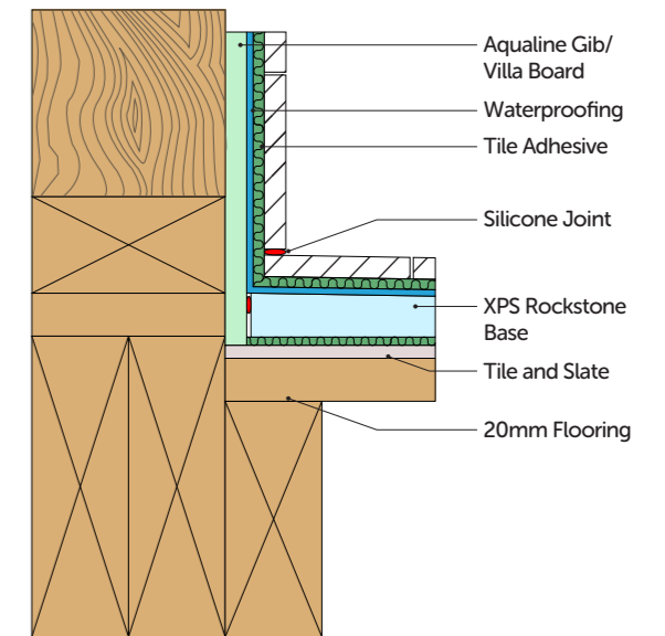
Rebate joists to required depth to suit base model Fix additional joists to support ply infill
