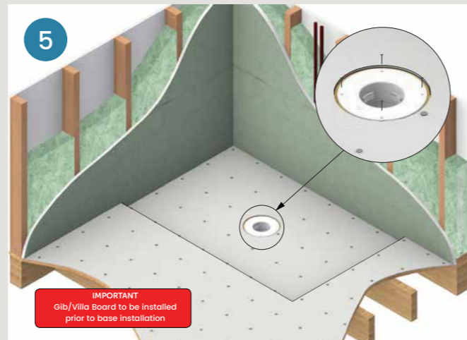
5 Glue PVC Flange to drain. Install tile & slate, ensuring 6mm clearance around LM flange. Install Gib/Villa board walls
