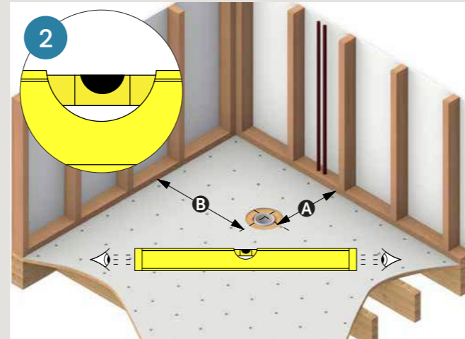
Lay 6mm Tile & Slate/Compressed Sheet over sub floor, cut circular clearance hole for LM Flange. Floor MUST be level
