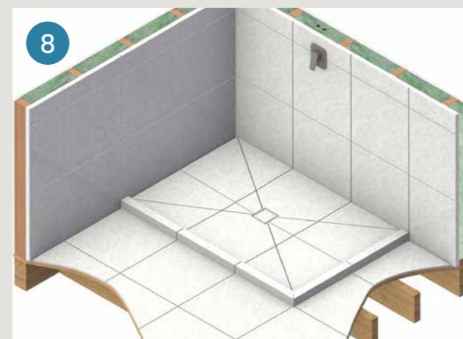
Tile walls and base. Grout and silicone seal all corner joints. Tile centre waste insert
